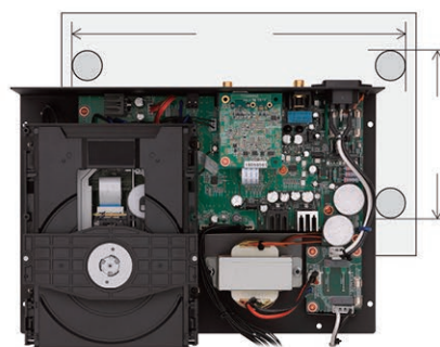
Internal configuration
