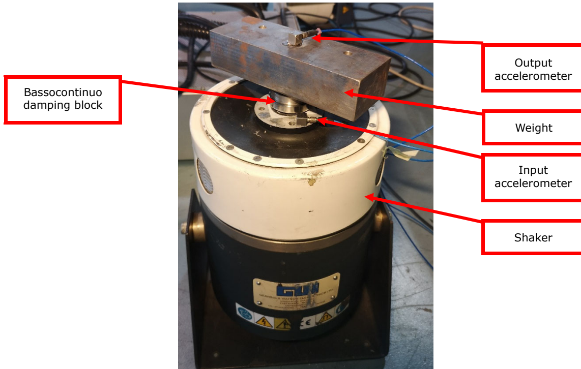
Figure 1. Test setup.
